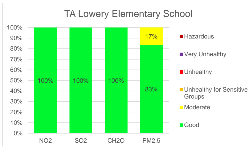
Figure 10: TALES AQI Distribution Summary – January through December 2021
