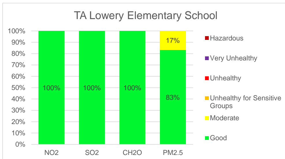
Figure 9: TALES AQI Distribution Summary — October through December 2021
