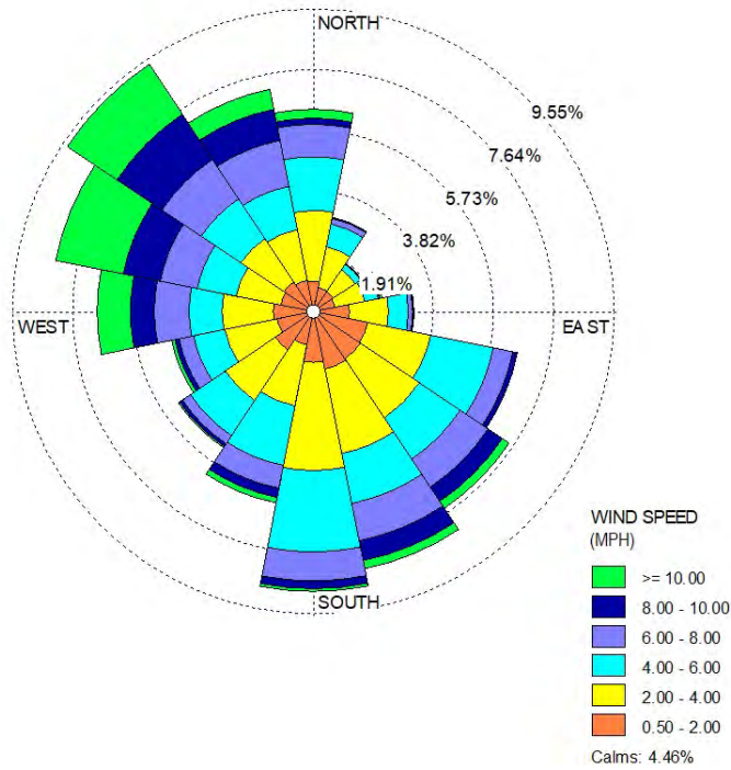
Figure 15: January through December 2021 Wind Rose
