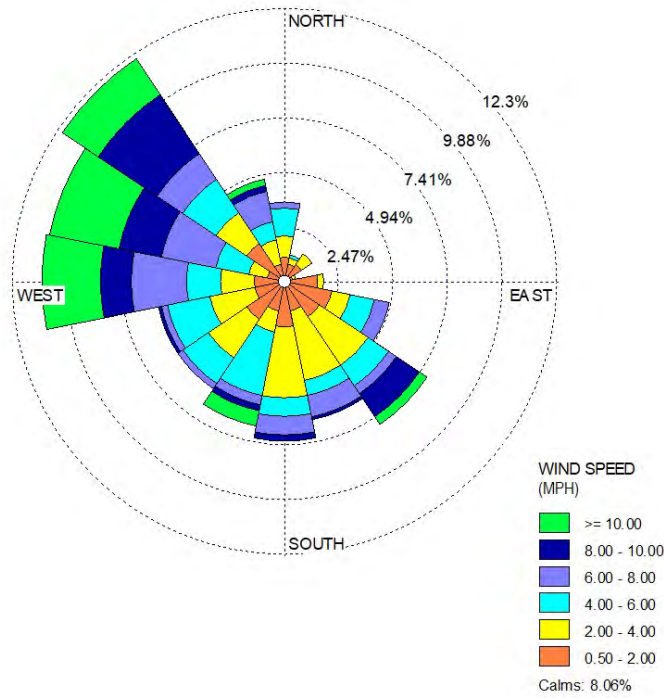
Figure 12: November 2021 Wind Rose
