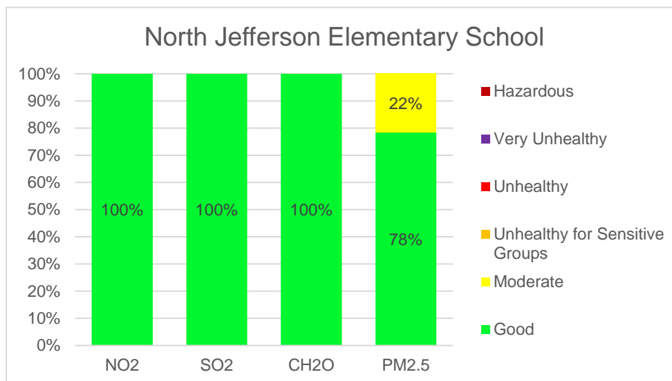
Figure 7: NJES AQI Distribution Summary — October through December 2021
