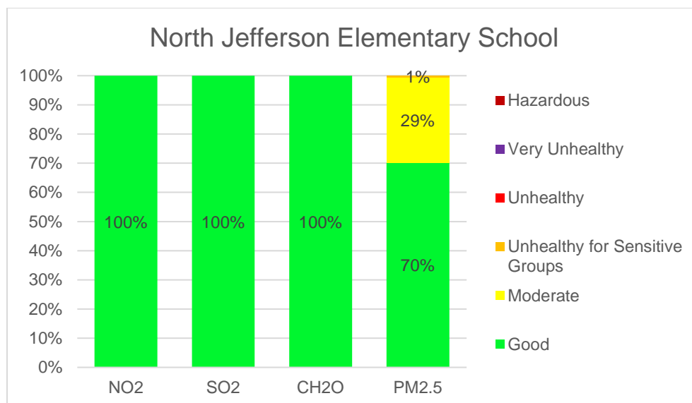
Figure 8: NJES AQI Distribution Summary – January through December 2021
