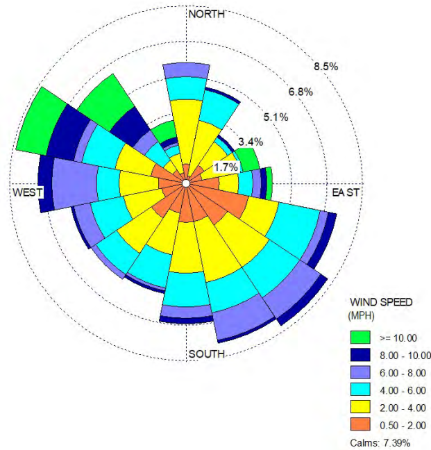
Figure 11: October 2021 Wind Rose
