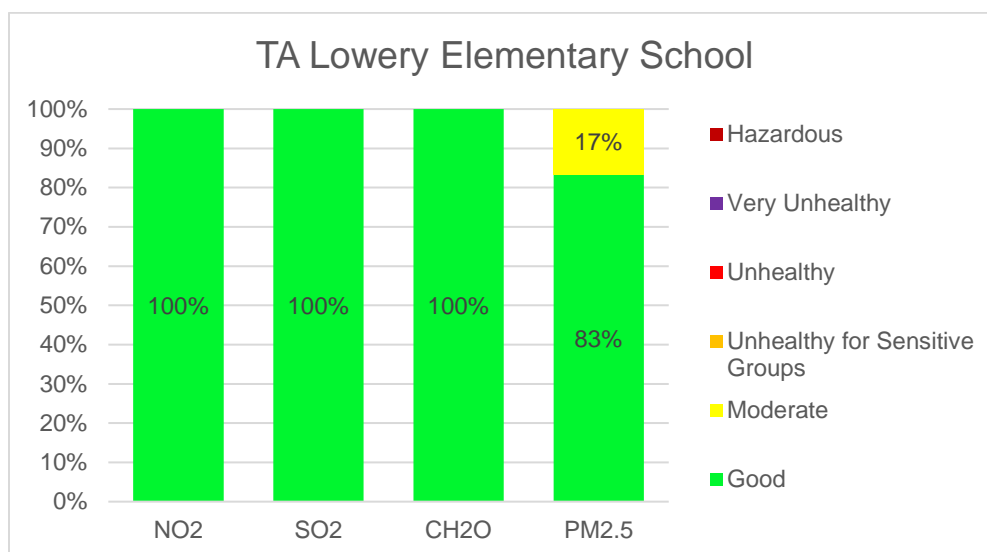
Figure 2: TALES AQI Distribution Summary — October through December 2021
