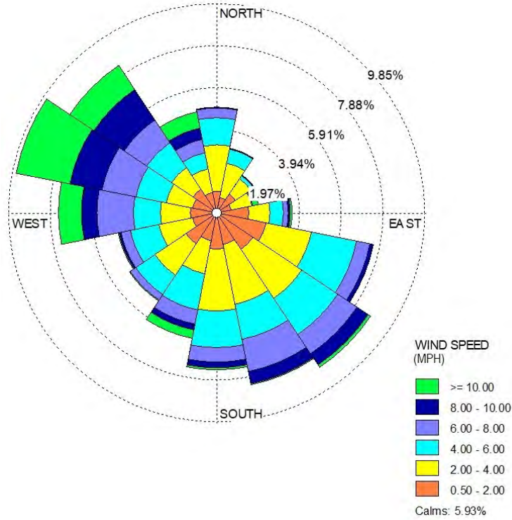
Figure 14: October through December 2021 Wind Rose
