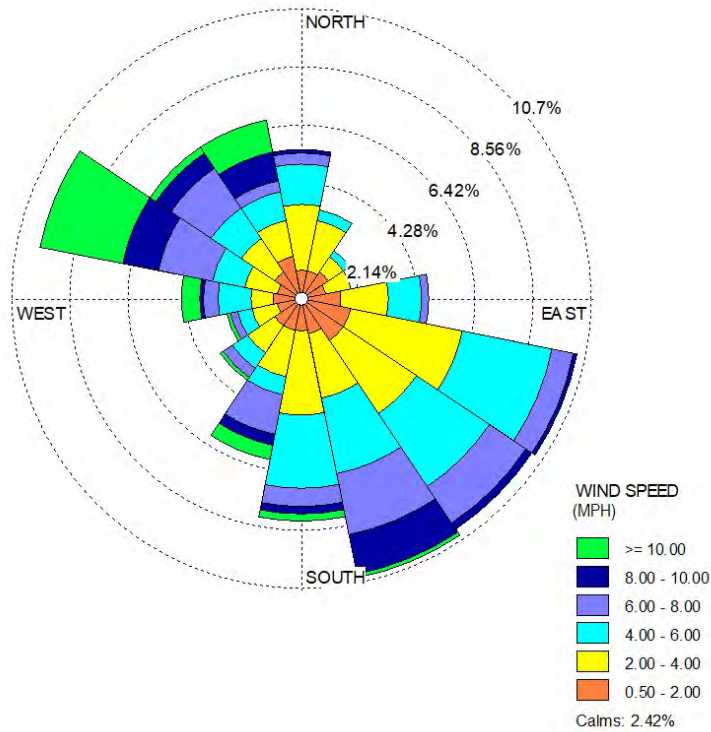
Figure 13: December 2021 Wind Rose
