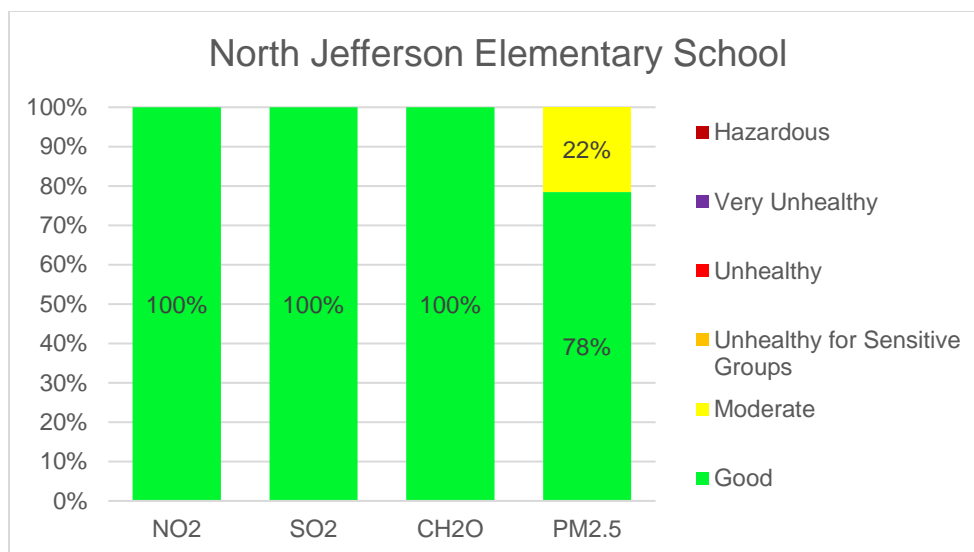
Figure 1: NJES AQI Distribution Summary — October through December 2021
