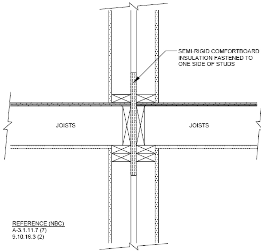
FIRE STOPPING DETAIL (CONCEALED SPACES)
